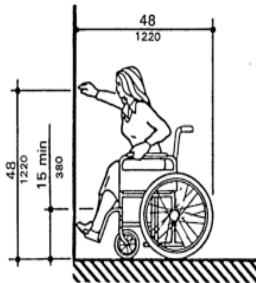
(a) High Forward Reach Limit
