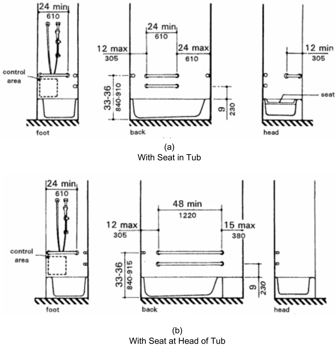
Fig. 34 Grab Bars at Bath Tubs
