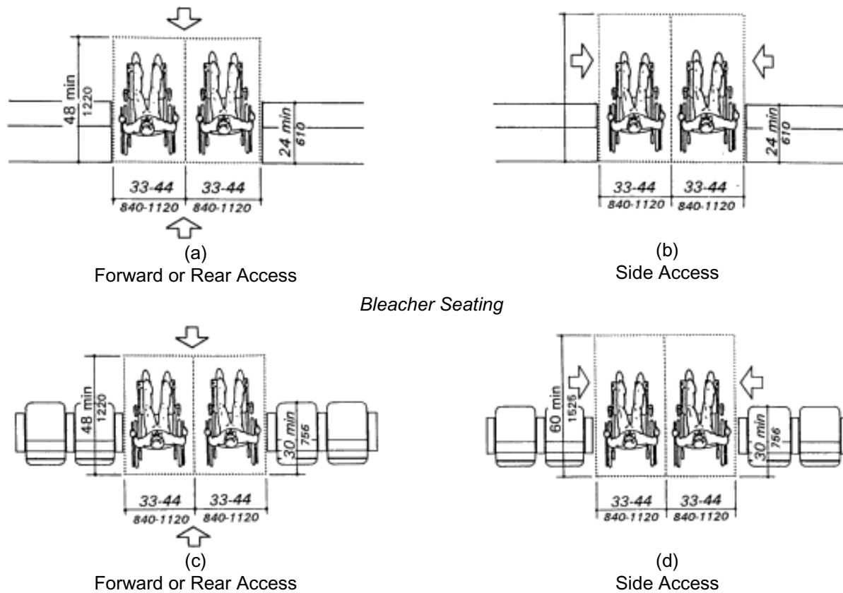
Fig. 46 Space Requirements for Wheelchair Seating Spaces in Series
