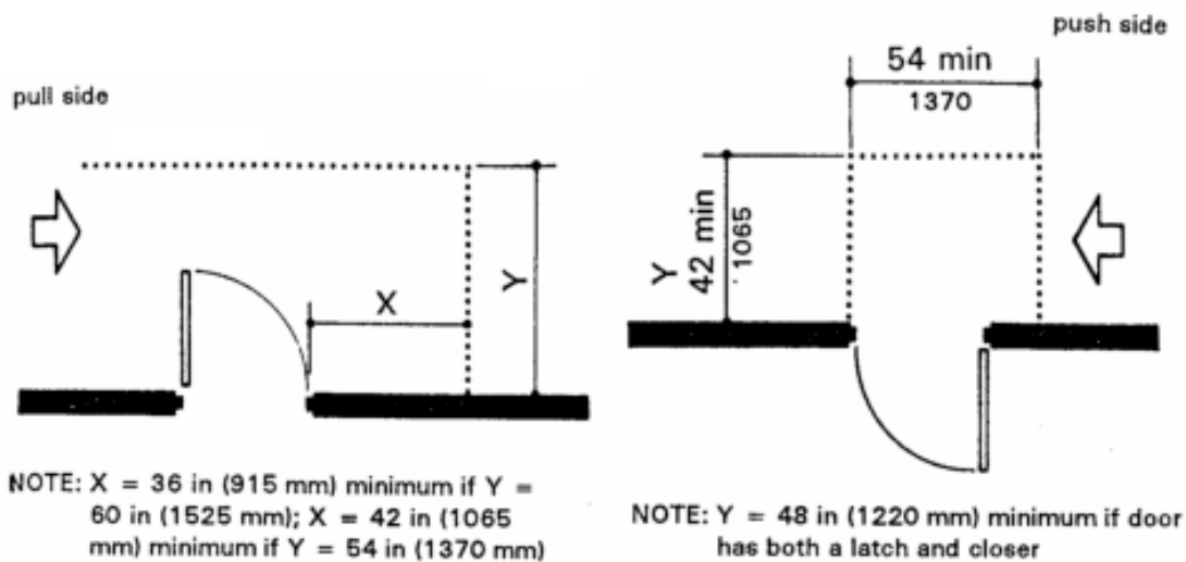
(b) Hinge Side Approaches Swinging Doors
