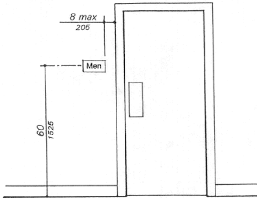
Fig. 43 (e) Signage Mounting Location and Height
