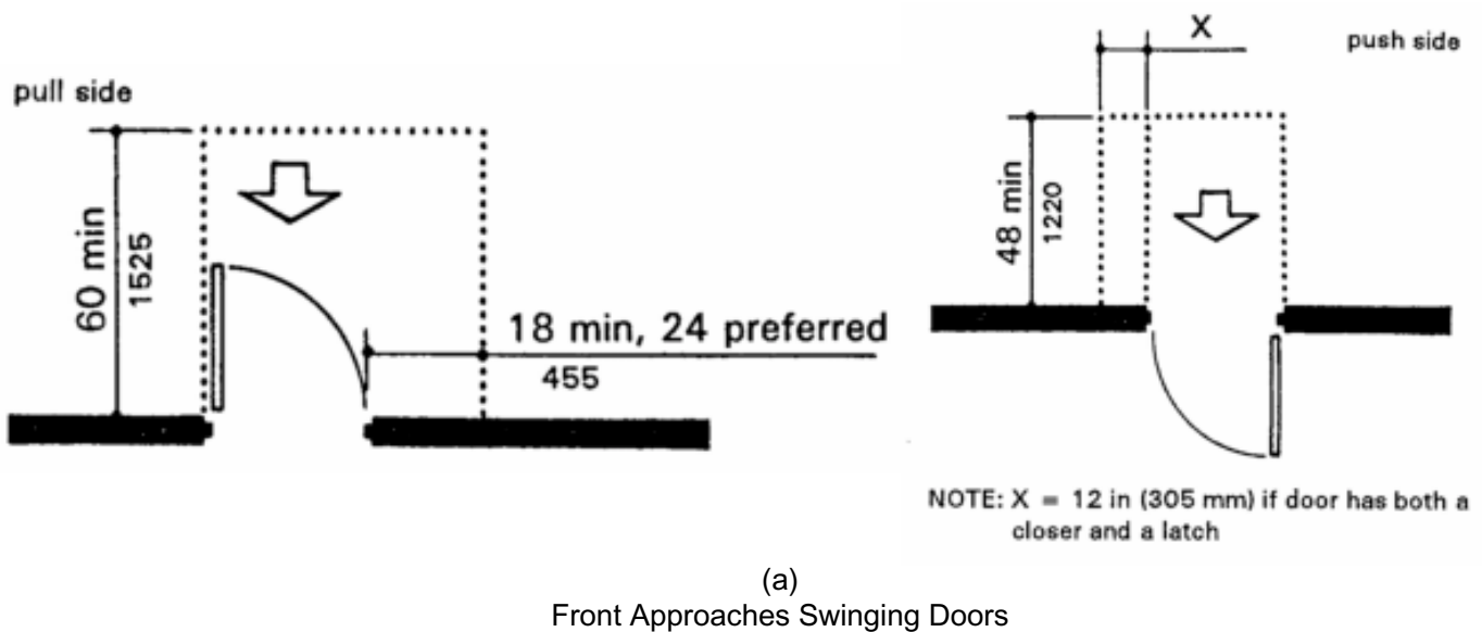
Fig. 24 Clear Doorway Width and Depth
