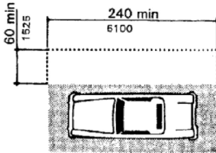
Fig. 10 Access Aisle at Passenger Loading Zones
