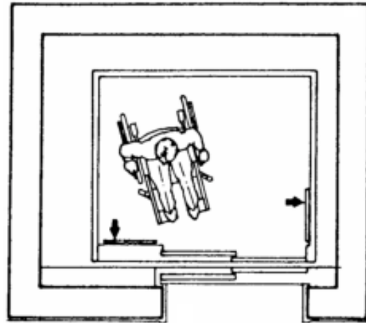
(d) Alternate Locations of Panels with Side Opening Door
