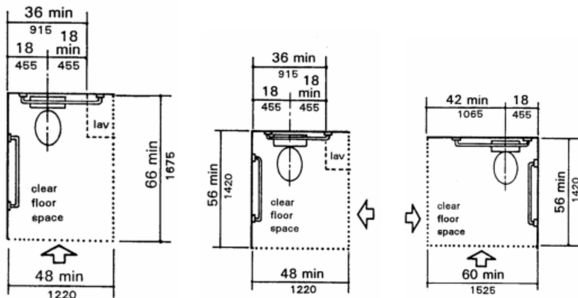
Fig. 28 Clear Floor Space at Water Closets
