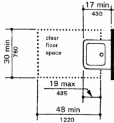
Fig. 32 Clear Floor Space for Lavatories
