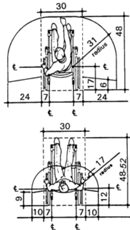
Fig. A2 Space Needed for a Smooth U-Turn in a Wheelchair
