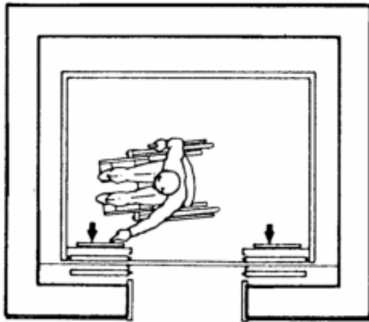
(c) Alternate Locations of Panels with Center Opening Door
