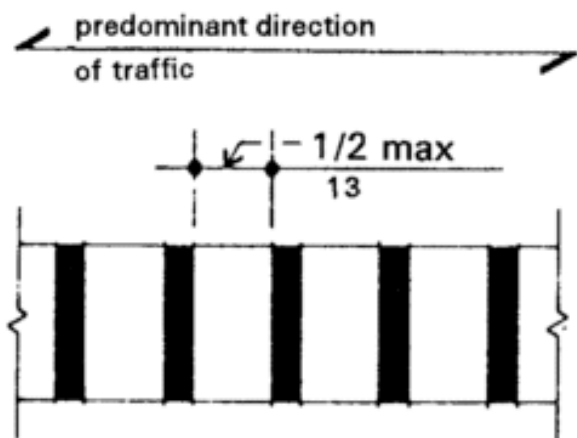
Fig. 8(g) Gratings
