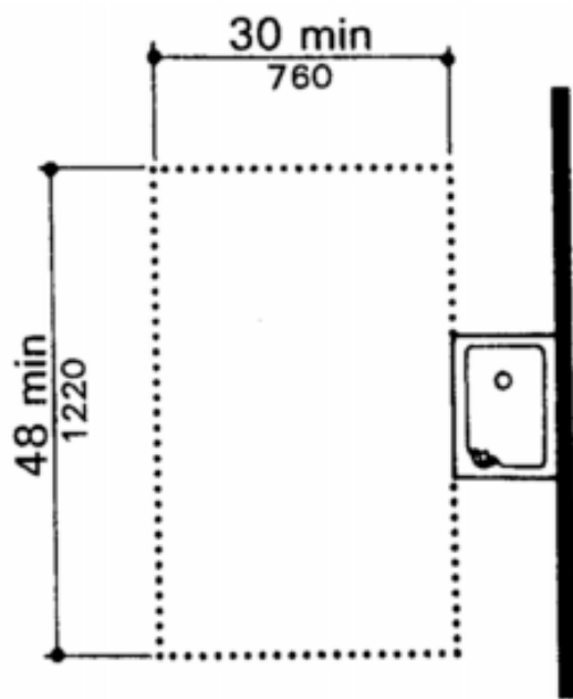
(c) Free-Standing fountain or Cooler
