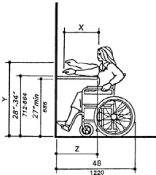
(a) High Forward Reach Limit
